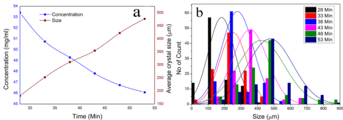
Figure 6. Solution concentration and average crystal size of a) SS-1.18 b) Crystal size distribution of SS-1.18.
