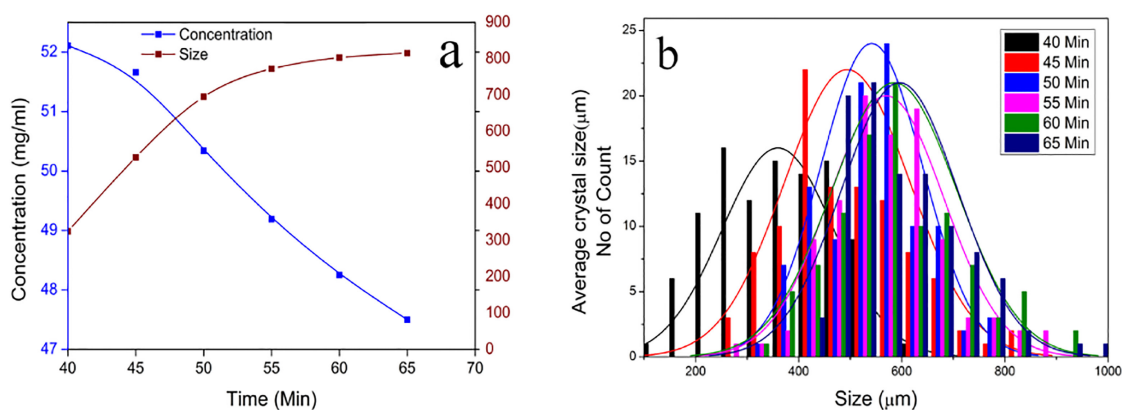
Figure 5. Solution concentration and average crystal size of a) SS-1.16 b) Crystal size distribution of SS-1.16.
