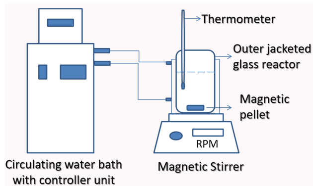
Figure 1. Schematic representation of Experimental Setup.
